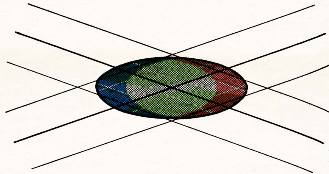
FIGURE Q9b.—Ellipse of uncertainty
