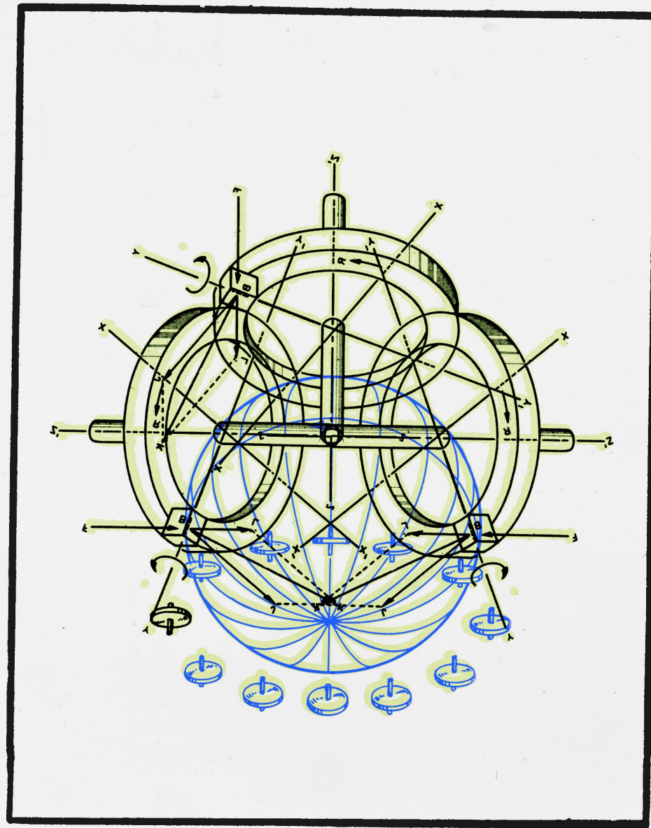
FIGURE 1513b.—Optical bubble sextant.
